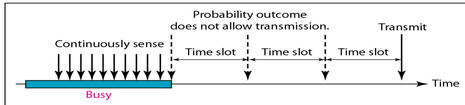
c. p-persistent
